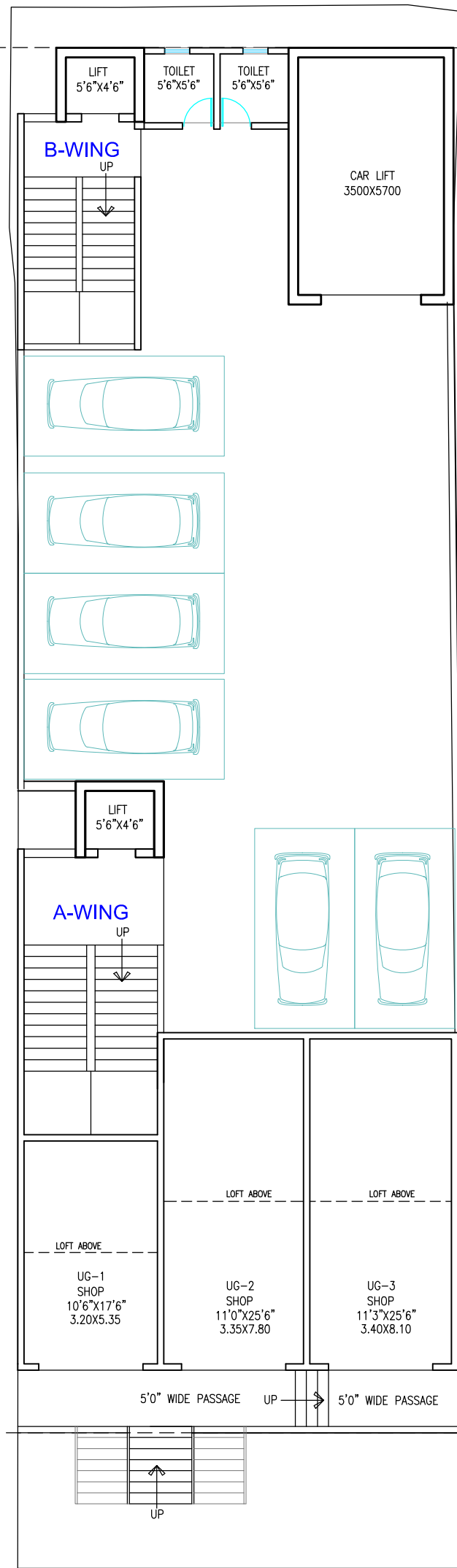
<<< ROAD >>> UPPER GROUND FLOOR PLAN
