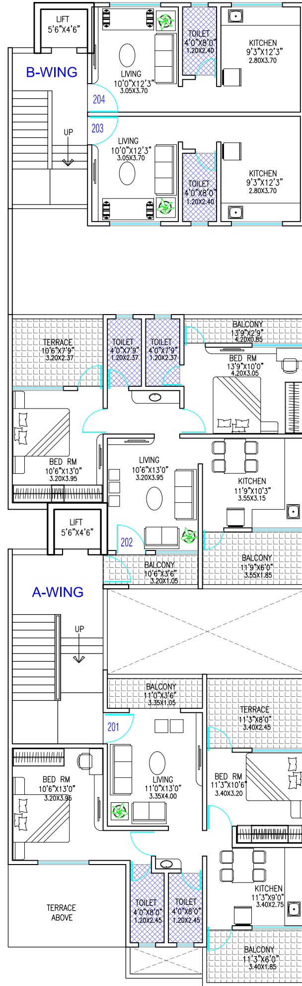
2nd FLOOR PLAN
